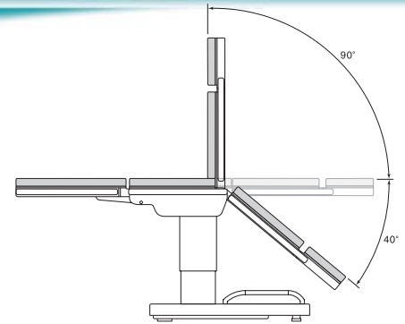
Back Up 90° Back Down 40°
