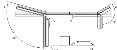
Head Up 30° Head Down 90° Leg Up 15° Leg Down 90°
